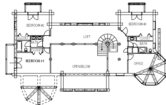
Second Floor Plan LIVING AREA: 1541 sqft
